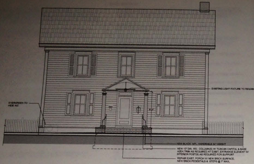
1 EAST ELEVATION SCALE: 1/4"=1'-0"
